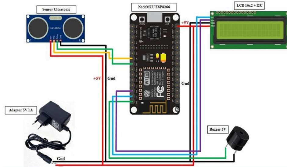
Fig 1. Schematic Circuit
