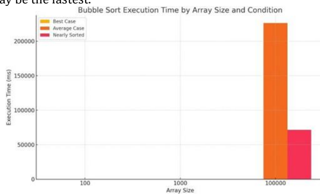
Fig. 3. Bubble sort
